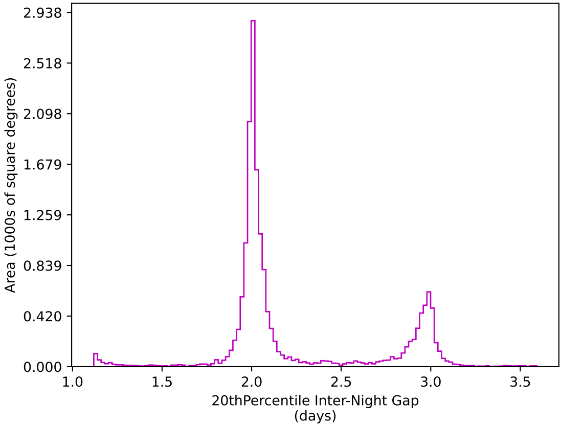
ddf_acor_sf15_lsf20_lsr20_v3.4_10yrs WFD z band: 20thPercentile Inter-Night Gap
