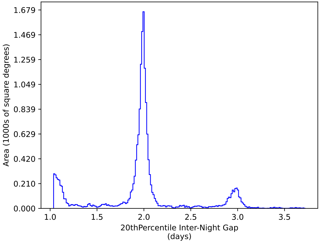
ddf_acor_sf15_lsf20_lsr20_v3.4_10yrs WFD y band: 20thPercentile Inter-Night Gap
