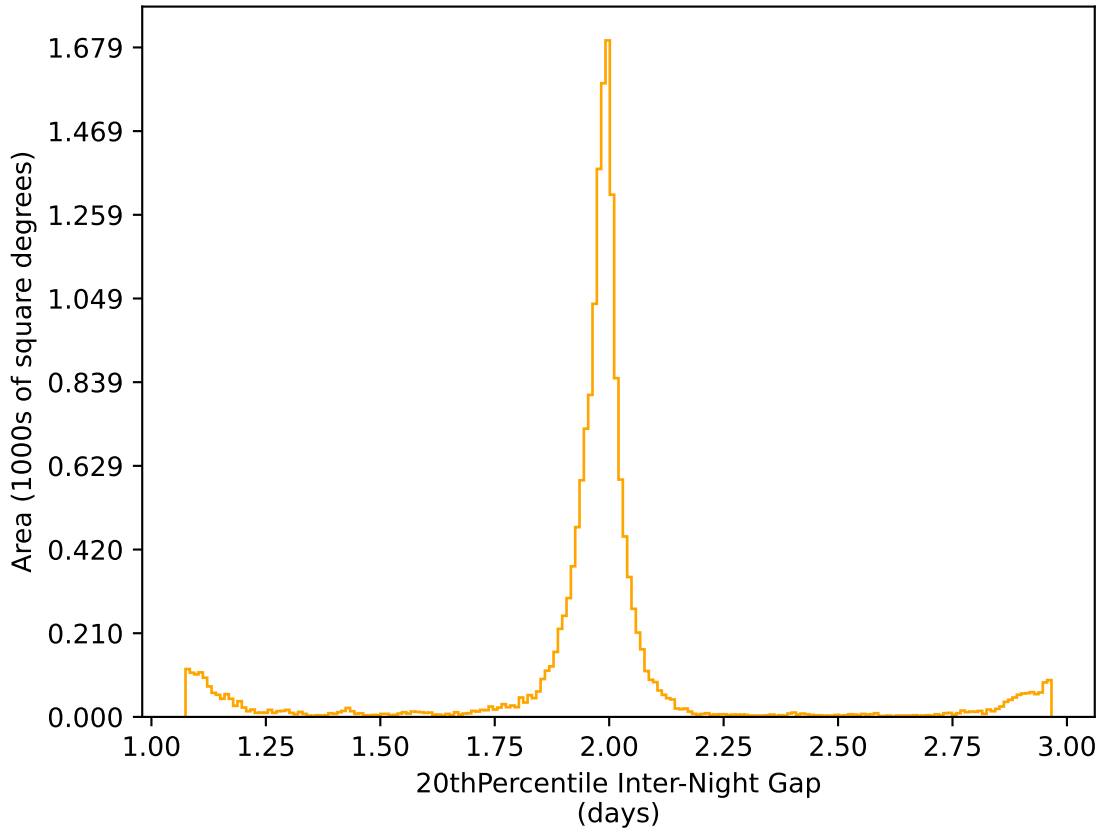
ddf_acor_sf15_lsf20_lsr20_v3.4_10yrs WFD r band: 20thPercentile Inter-Night Gap
