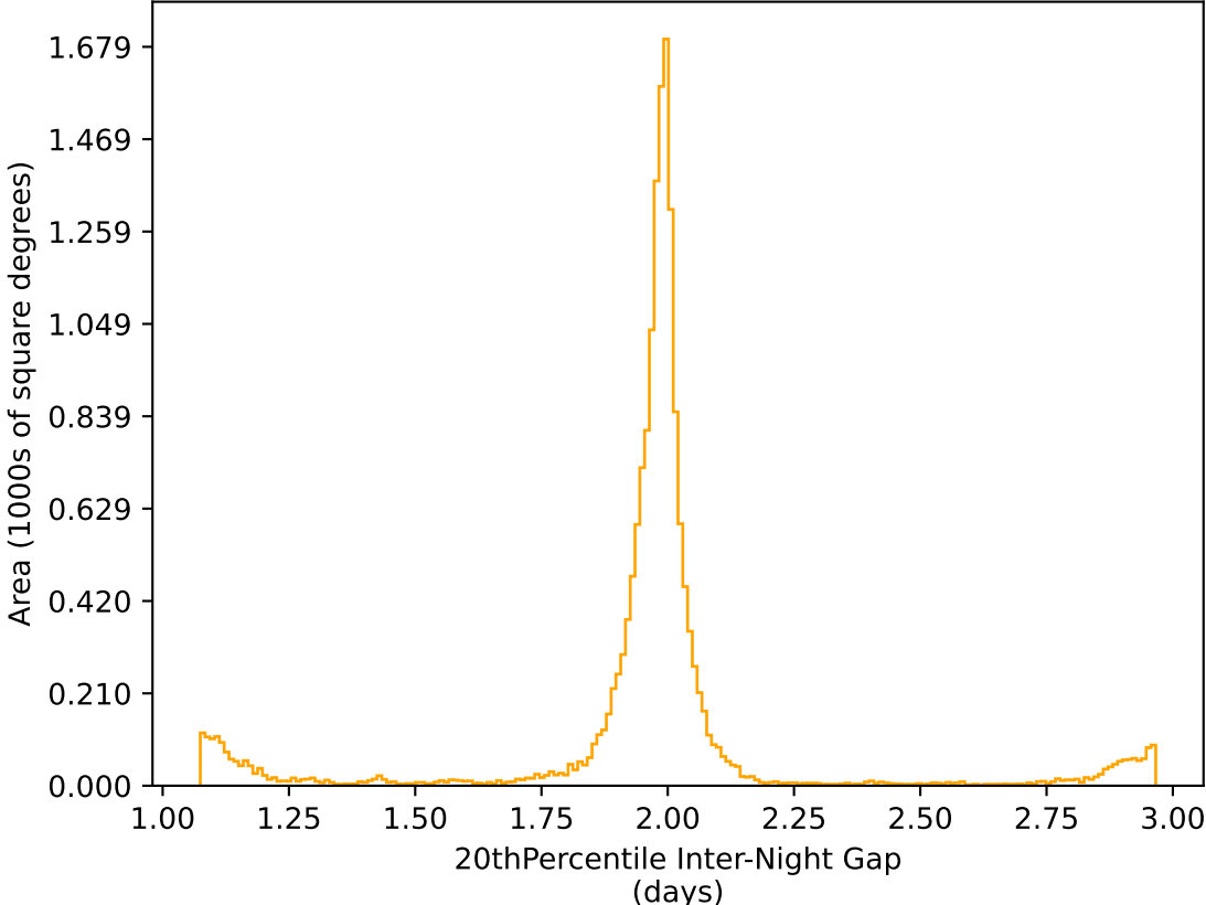
ddf_acor_sf15_lsf20_lsr20_v3.4_10yrs WFD r band: 20thPercentile Inter-Night Gap
