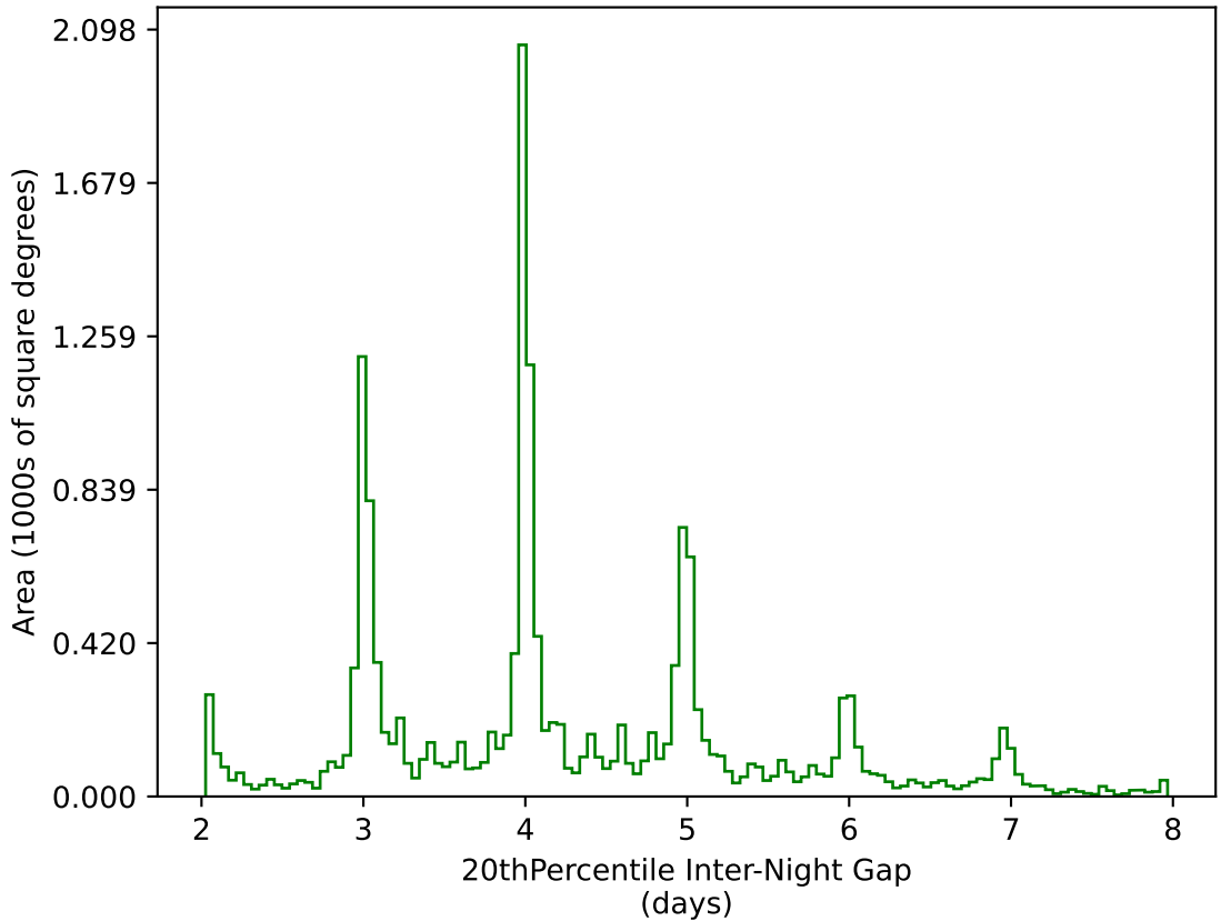
ddf_acor_sf15_lsf20_lsr20_v3.4_10yrs WFD g band: 20thPercentile Inter-Night Gap
