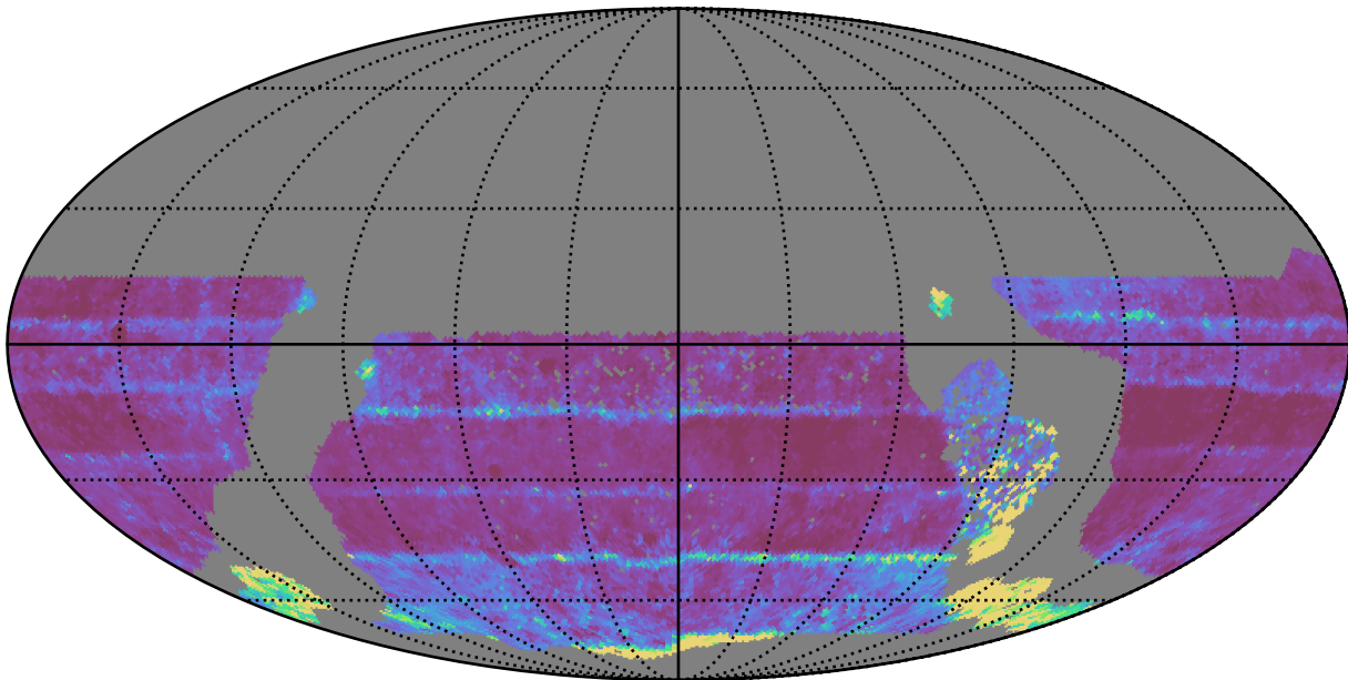
ddf_acor_sf15_lsf20_lsr20_v3.4_10yrs WFD all bands: 20thPercentile Inter-Night Gap
