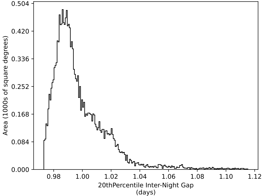
ddf_acor_sf15_lsf20_lsr20_v3.4_10yrs WFD all bands: 20thPercentile Inter-Night Gap
