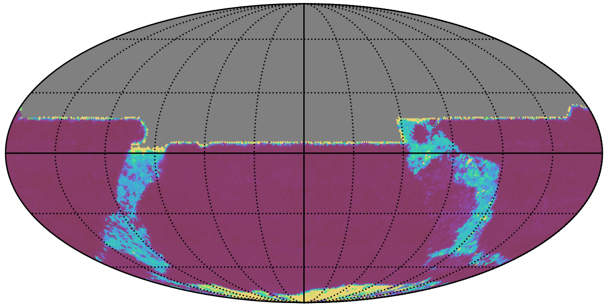
ddf_acor_sf15_lsf20_lsr20_v3.4_10yrs All sky y band: 20thPercentile Inter-Night Gap
