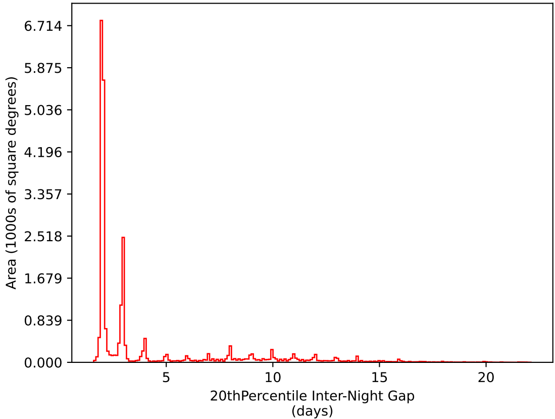
ddf_acor_sf15_lsf20_lsr20_v3.4_10yrs All sky i band: 20thPercentile Inter-Night Gap
