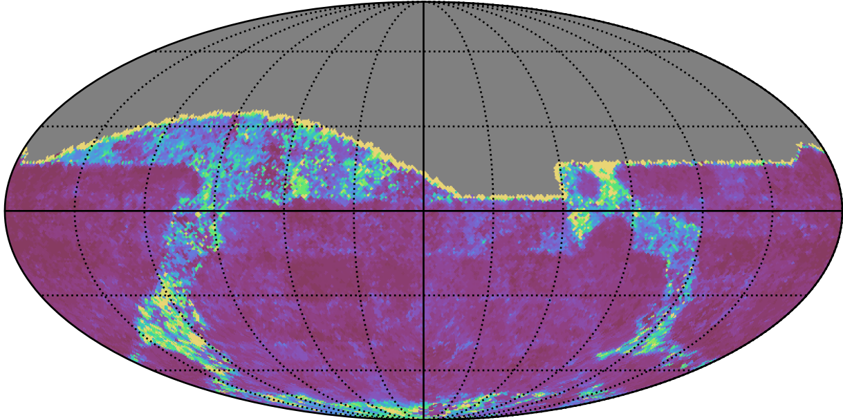
ddf_acor_sf15_lsf20_lsr20_v3.4_10yrs All sky g band: 20thPercentile Inter-Night Gap
