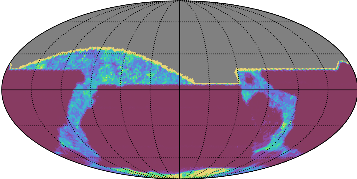
ddf_acor_sf15_lsf20_lsr20_v3.4_10yrs All sky all bands: 20thPercentile Inter-Night Gap
