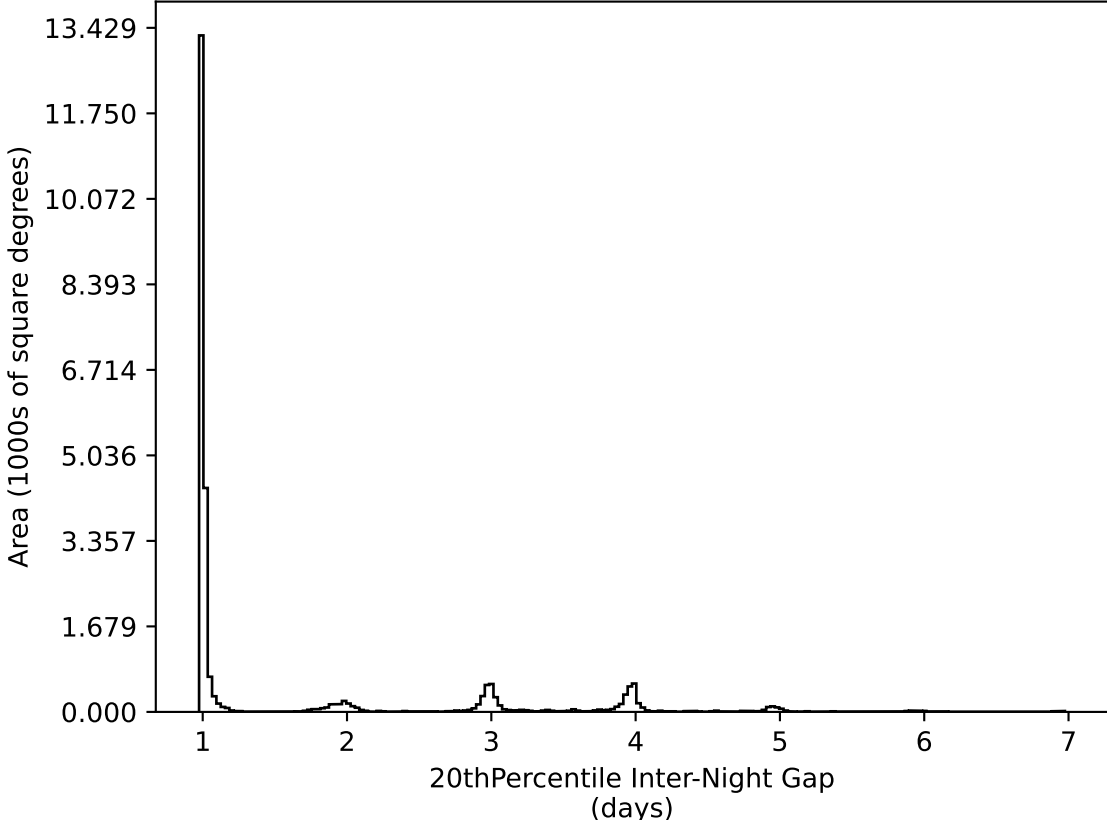
ddf_acor_sf15_lsf20_lsr20_v3.4_10yrs All sky all bands: 20thPercentile Inter-Night Gap
