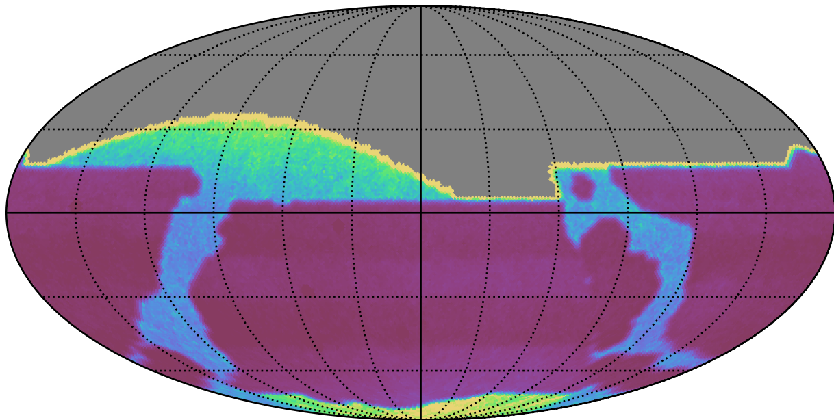
ddf_acor_sf15_lsf20_lsr20_v3.4_10yrs : properMotion
