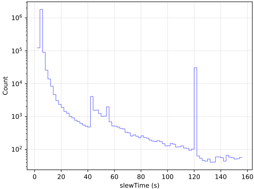
ddf_acor_sf15_lsf20_lsr20_v3.4_10yrs All visits: Slew Time Histogram
