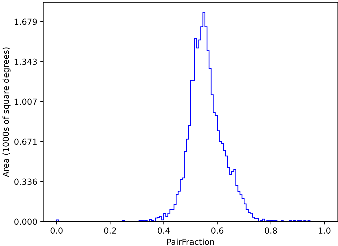
ddf_acor_sf15_lsf20_lsr20_v3.4_10yrs (g or r or i): PairFraction
