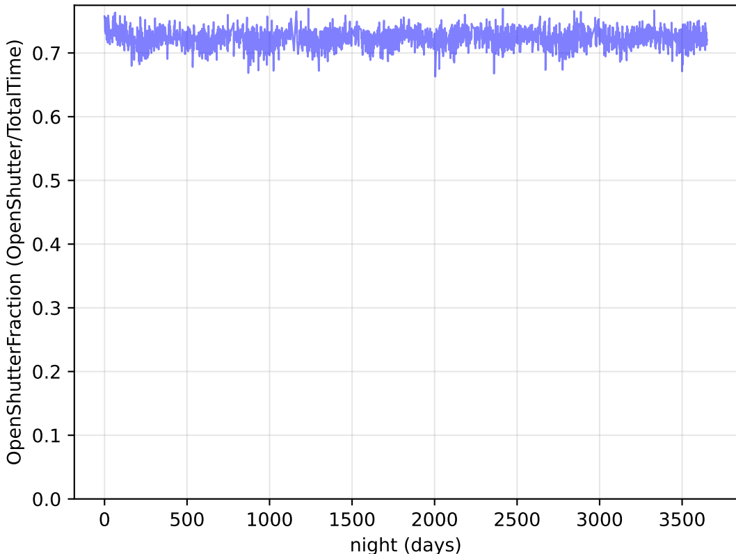
ddf_acor_sf15_lsf20_lsr20_v3.4_10yrs : OpenShutterFraction
