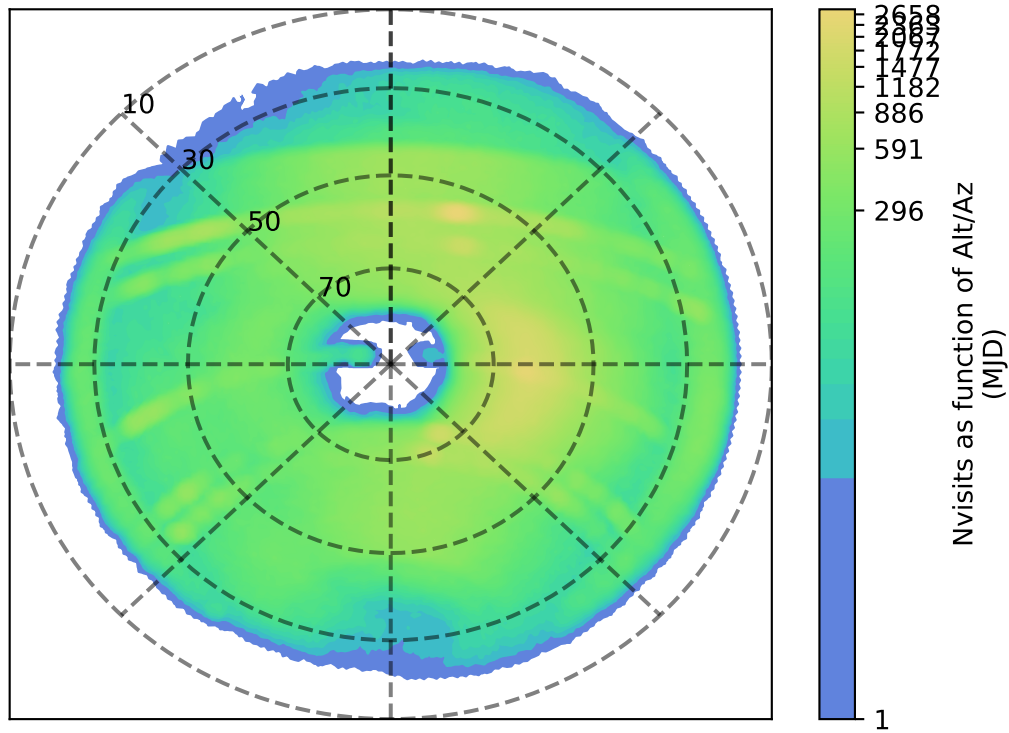
ddf_acor_sf15_lsf20_lsr20_v3.4_10yrs z: Nvisits as function of Alt/Az
