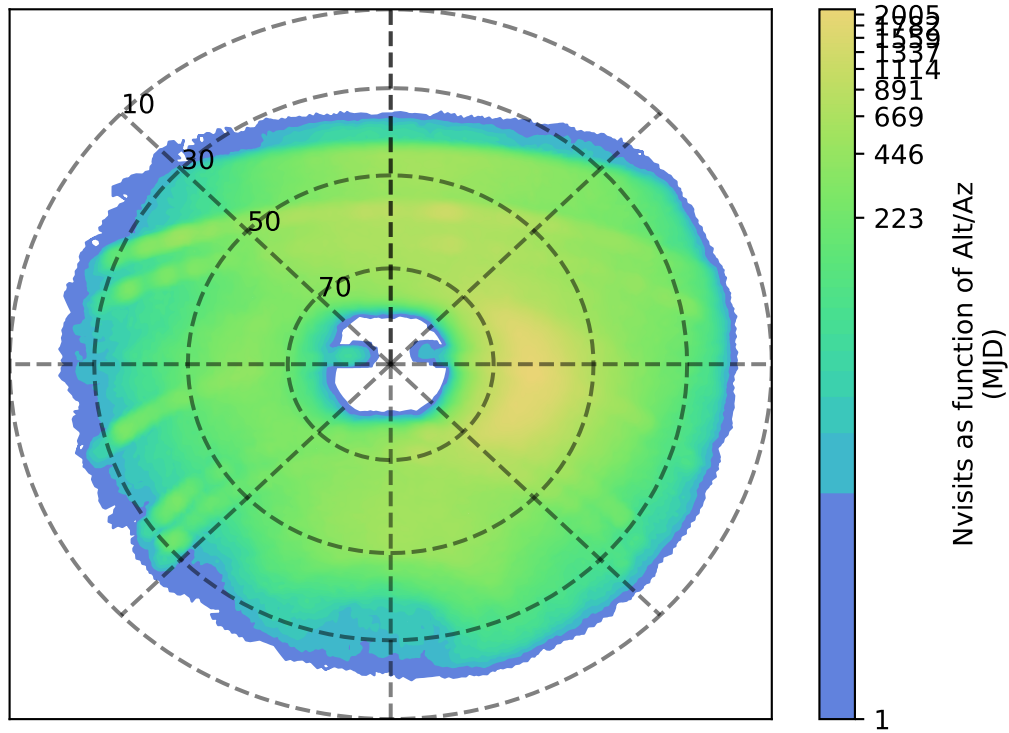
ddf_acor_sf15_lsf20_lsr20_v3.4_10yrs y: Nvisits as function of Alt/Az
