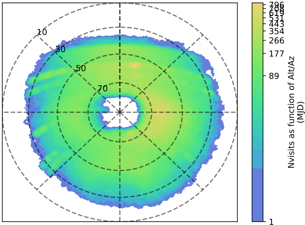
ddf_acor_sf15_lsf20_lsr20_v3.4_10yrs u: Nvisits as function of Alt/Az
