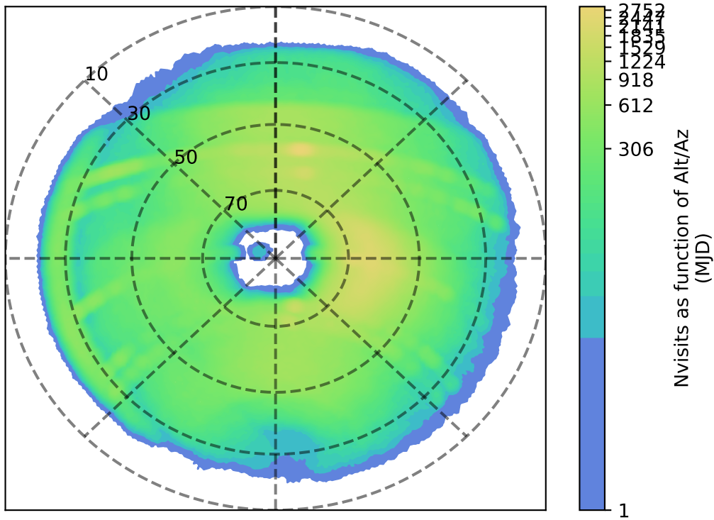
ddf_acor_sf15_lsf20_lsr20_v3.4_10yrs r: Nvisits as function of Alt/Az
