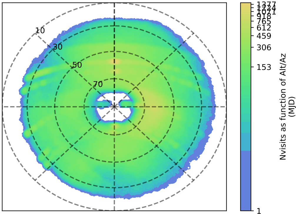
ddf_acor_sf15_lsf20_lsr20_v3.4_10yrs g: Nvisits as function of Alt/Az
