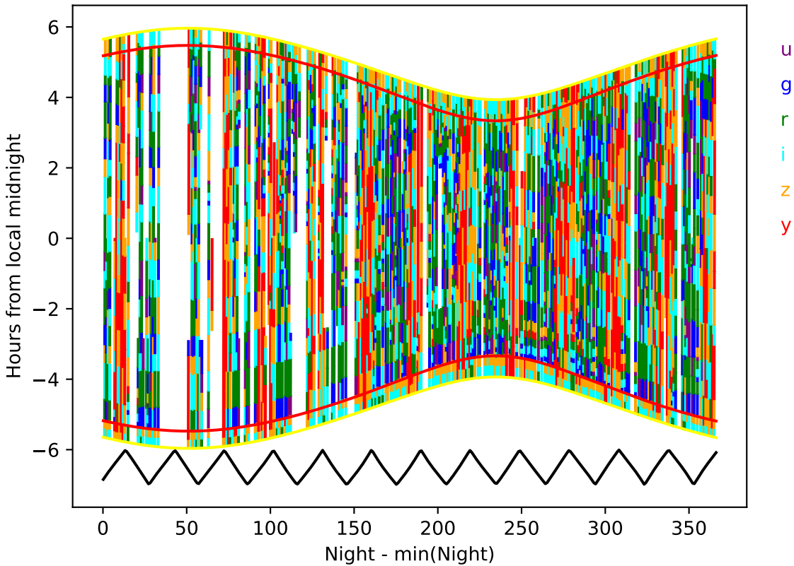
ddf_acor_sf15_lsf20_lsr20_v3.4_10yrs year 8-9: Hourglass
