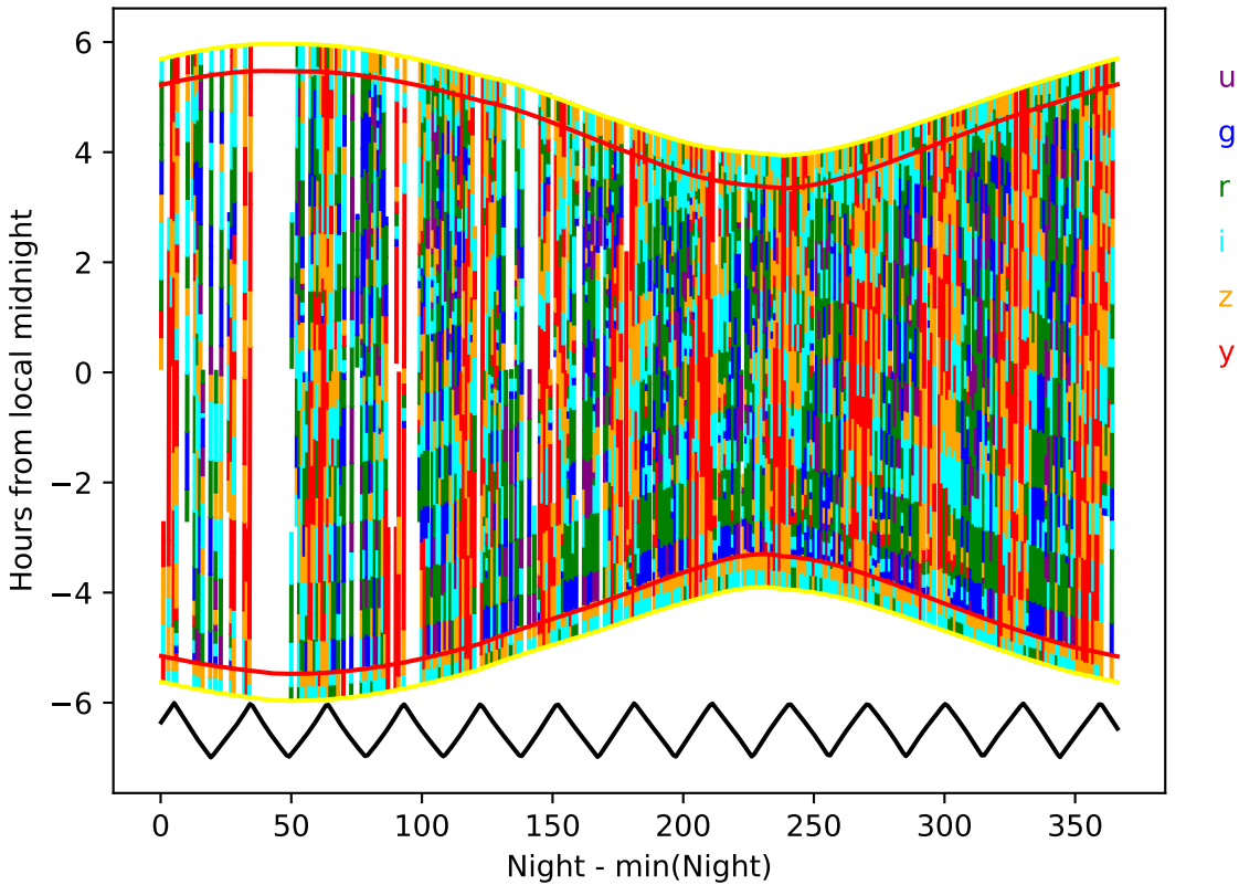
ddf_acor_sf15_lsf20_lsr20_v3.4_10yrs year 6-7: Hourglass
