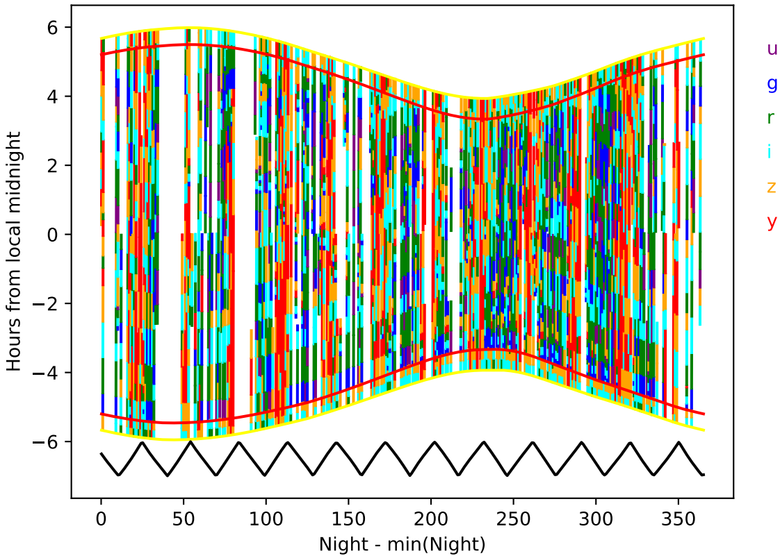
ddf_acor_sf15_lsf20_lsr20_v3.4_10yrs year 4-5: Hourglass
