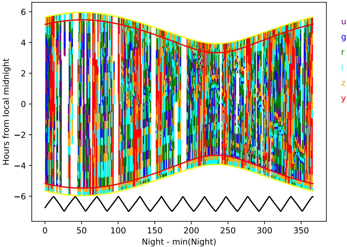
ddf_acor_sf15_lsf20_lsr20_v3.4_10yrs year 0-1: Hourglass
