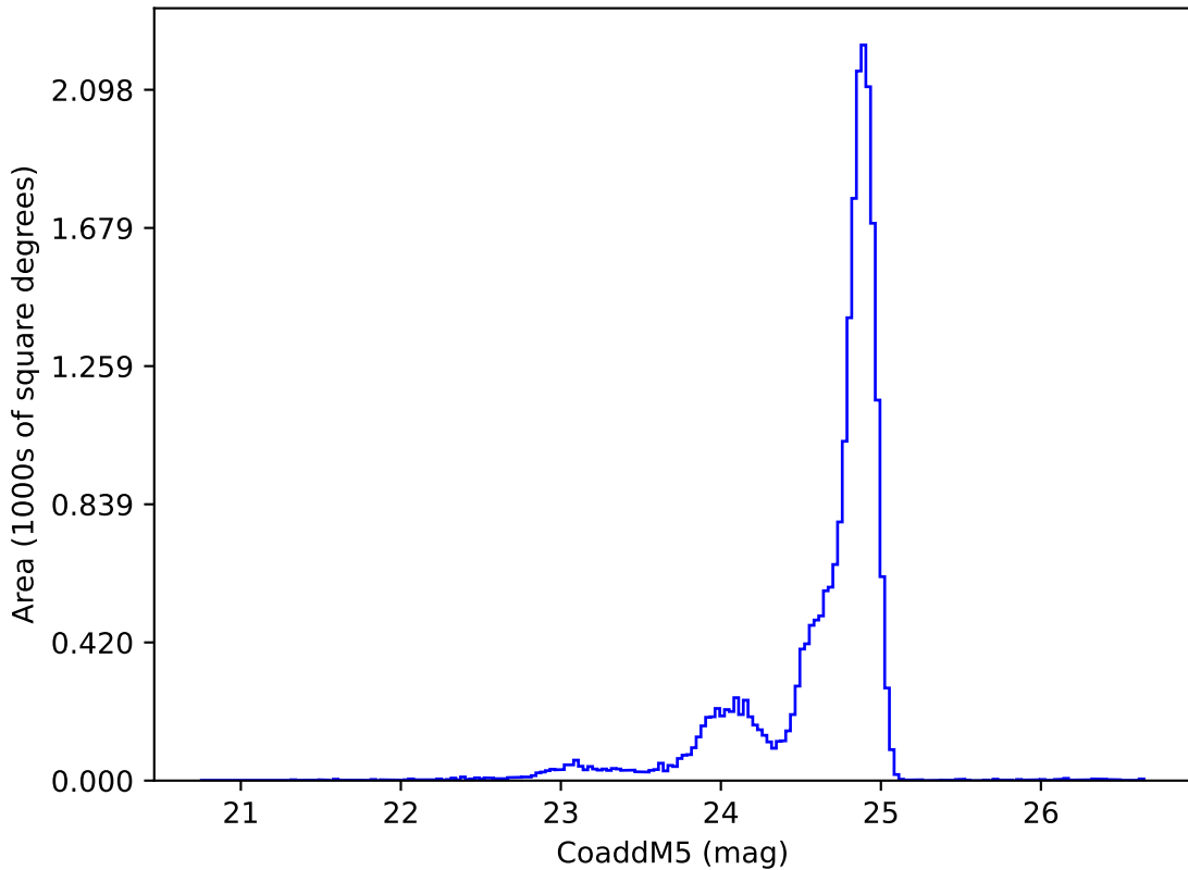
ddf_acor_sf15_lsf20_lsr20_v3.4_10yrs y: CoaddM5
