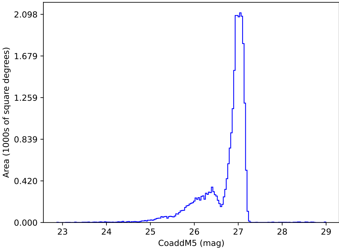
ddf_acor_sf15_lsf20_lsr20_v3.4_10yrs r: CoaddM5
