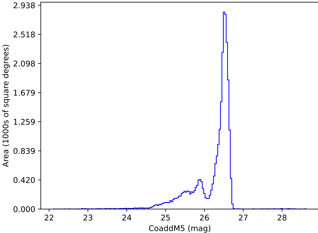
ddf_acor_sf15_lsf20_lsr20_v3.4_10yrs i: CoaddM5
