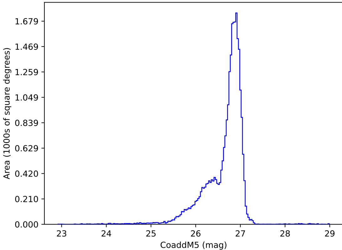
ddf_acor_sf15_lsf20_lsr20_v3.4_10yrs g: CoaddM5
