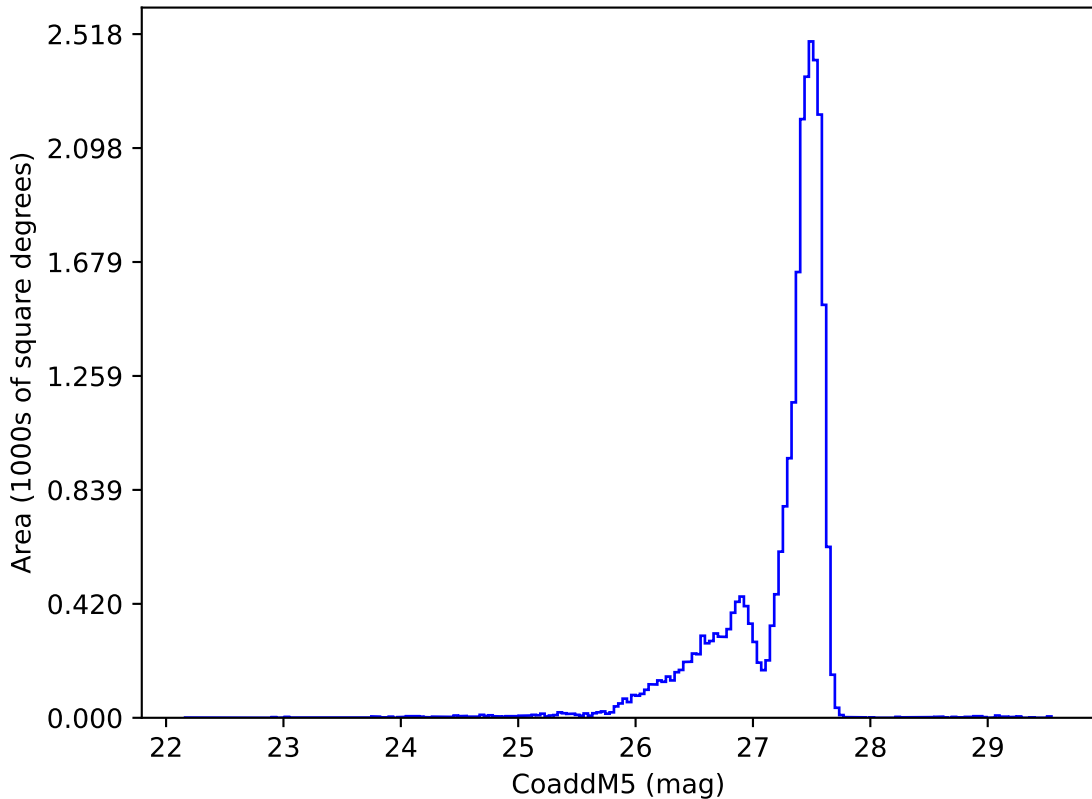
ddf_acor_sf15_lsf20_lsr20_v3.4_10yrs : CoaddM5
