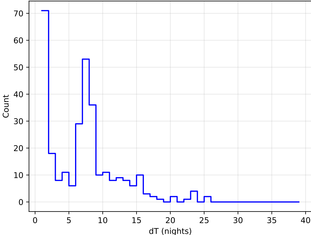
ddf_acor_sf15_lsf20_lsr20_v3.4_10yrs all bands: DD:XMM_LSS Delta Nights Histogram
