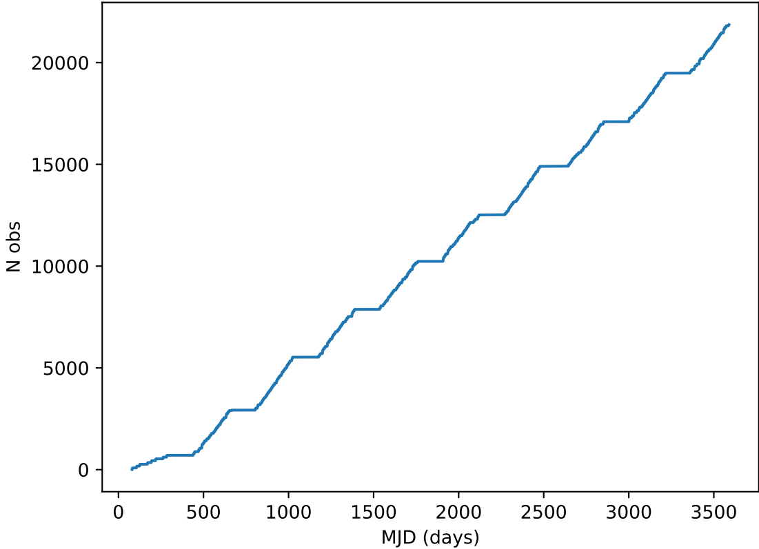
ddf_acor_sf15_lsf20_lsr20_v3.4_10yrs all bands: DD:XMM_LSS Cumulative NVisits
