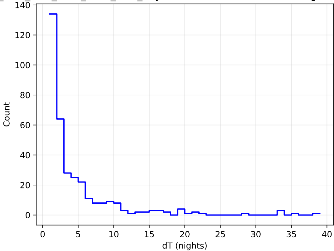
ddf_acor_sf15_lsf20_lsr20_v3.4_10yrs all bands: DD:WFD Delta Nights Histogram
