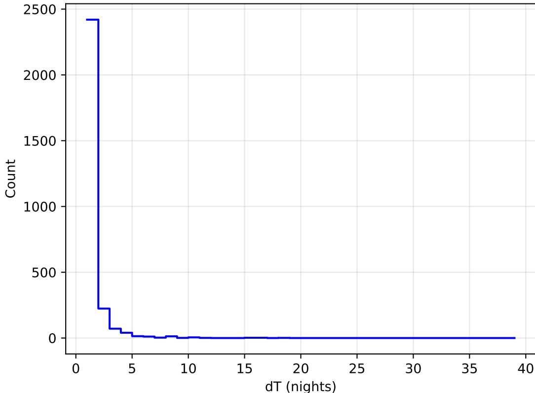
ddf_acor_sf15_lsf20_lsr20_v3.4_10yrs all bands: DD:WFD Delta Nights Histogram
