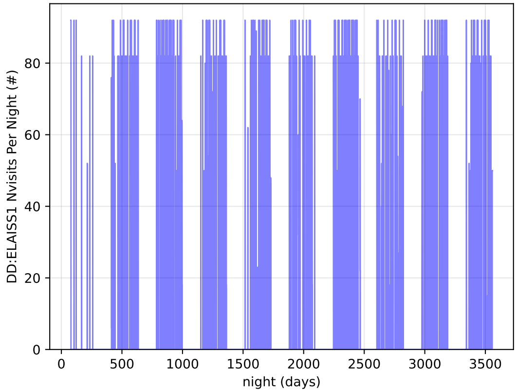
ddf_acor_sf15_lsf20_lsr20_v3.4_10yrs all bands: DD:ELAISS1 Nvisits Per Night
