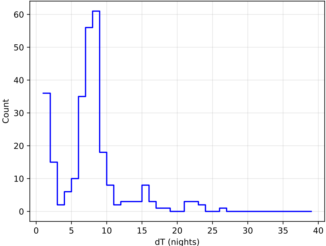
ddf_acor_sf15_lsf20_lsr20_v3.4_10yrs all bands: DD:ELAISS1 Delta Nights Histogram
