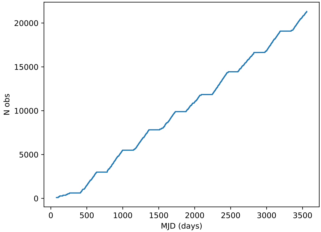
ddf_acor_sf15_lsf20_lsr20_v3.4_10yrs all bands: DD:ELAISS1 Cumulative NVisits
