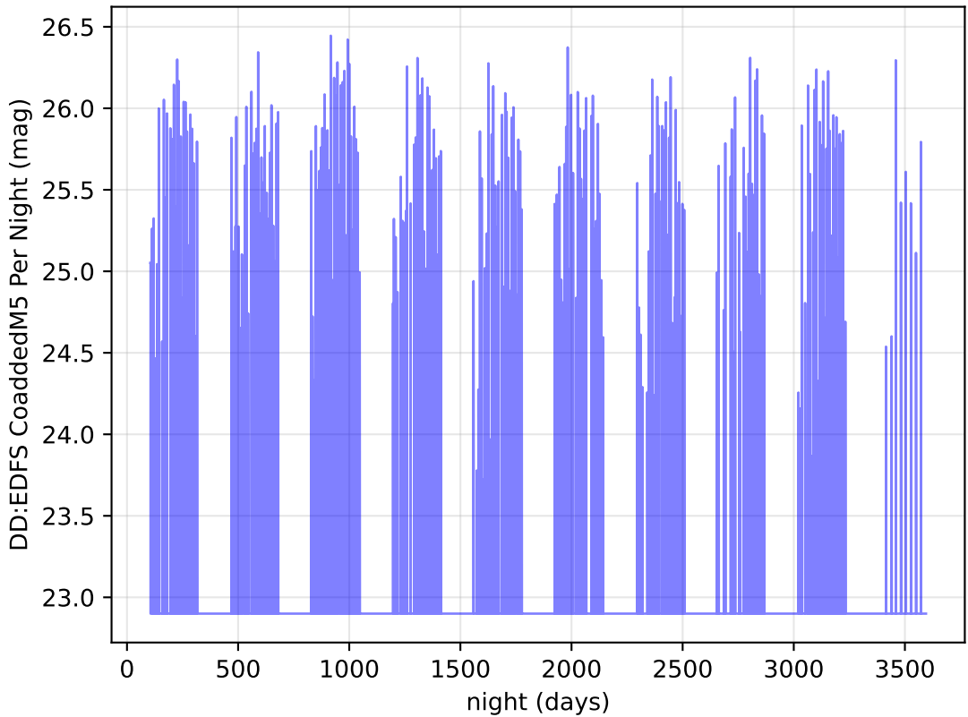
ddf_acor_sf15_lsf20_lsr20_v3.4_10yrs r band: DD:EDFS CoaddedM5 Per Night
