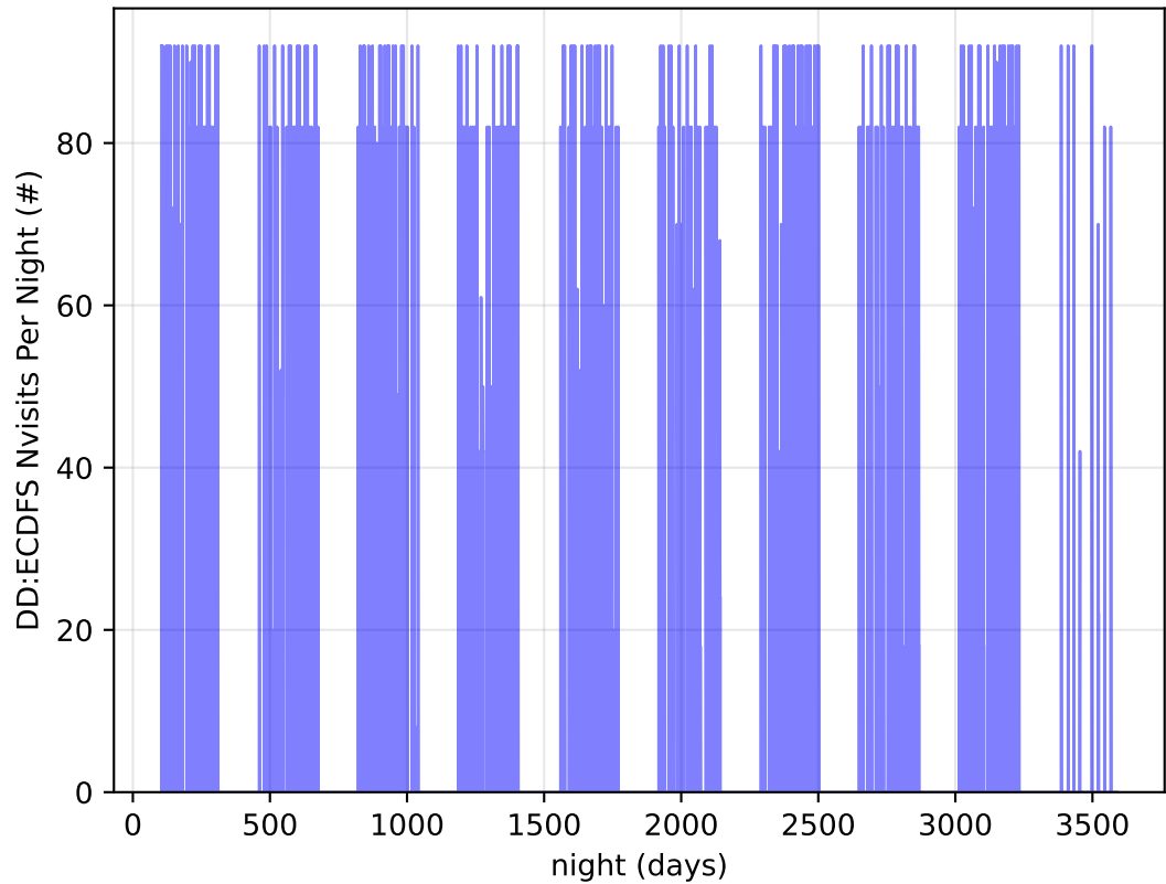
ddf_acor_sf15_lsf20_lsr20_v3.4_10yrs all bands: DD:ECDFS Nvisits Per Night
