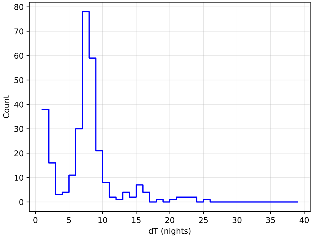
ddf_acor_sf15_lsf20_isr20_v3.4_10yrs all bands: DD:ECDFS Delta Nights Histogram
