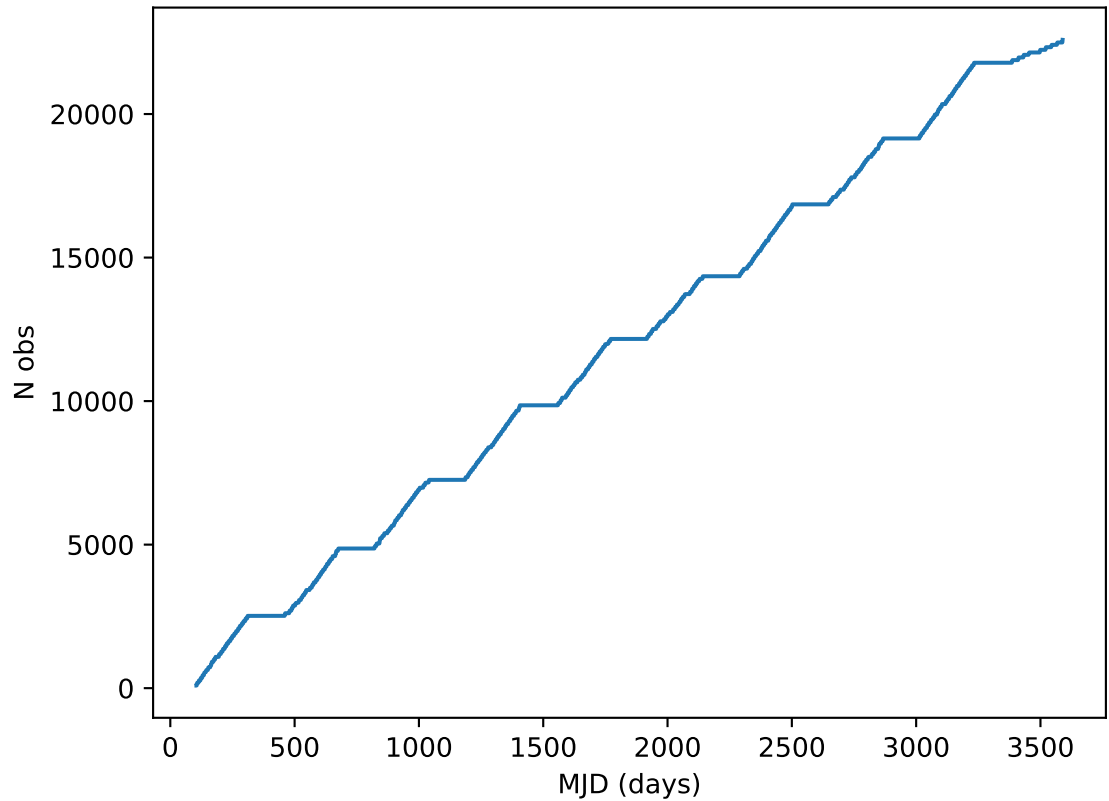
ddf_acor_sf15_lsf20_lsr20_v3.4_10yrs all bands: DD:ECDFS Cumulative NVisits
