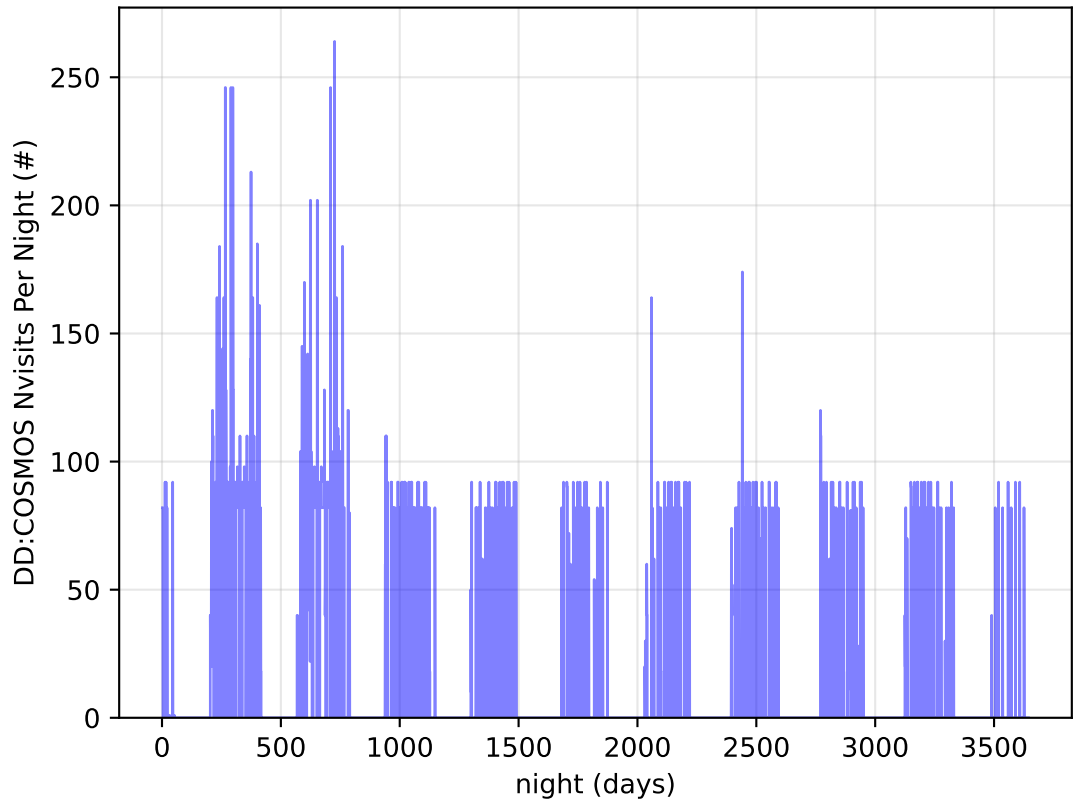
ddf_acor_sf15_lsf20_lsr20_v3.4_10yrs all bands: DD: COSMOS Nvisits Per Night
