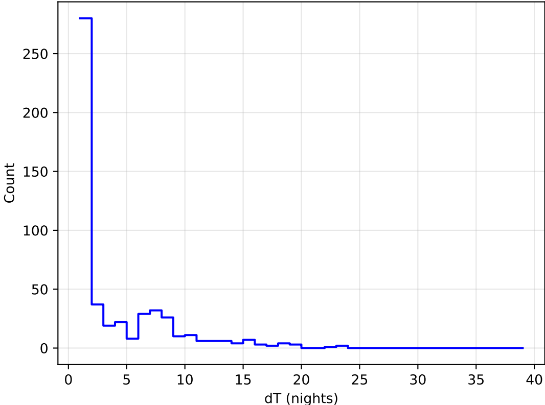
ddf_acor_sf15_lsf20_lsr20_v3.4_10yrs all bands: DD:COSMOS Delta Nights Histogram
