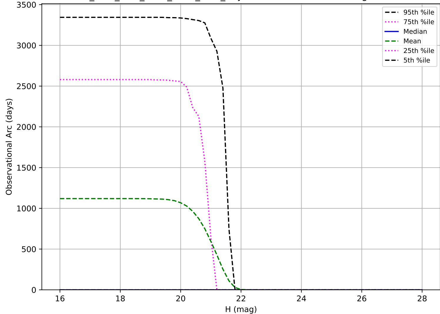
ddf_acor_sf15_lsf20_lsr10_v3.4_10yrs: Observational Arc Length Vatira
