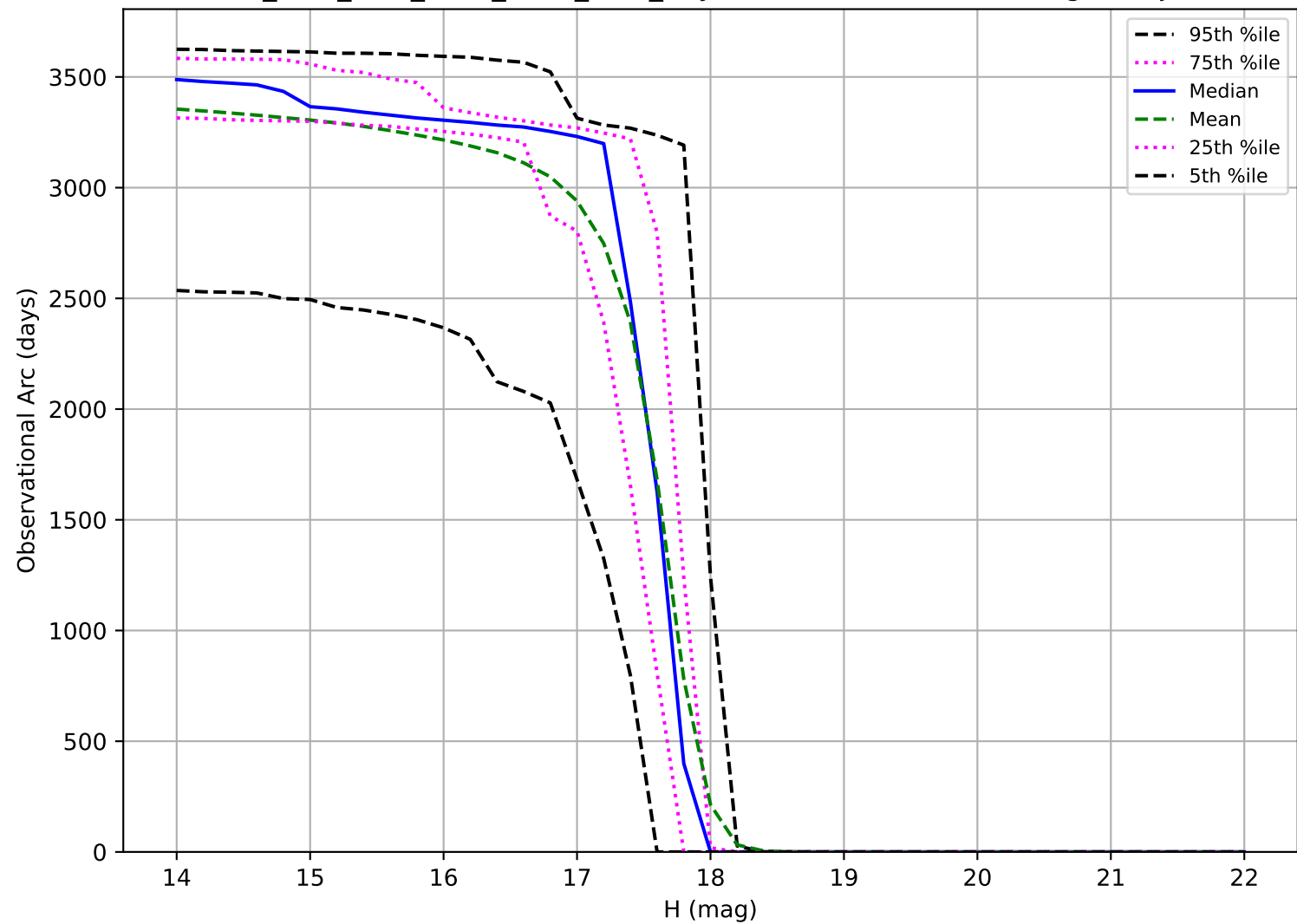
ddf_acor_sf15_lsf20_lsr10_v3.4_10yrs: Observational Arc Length Trojan
