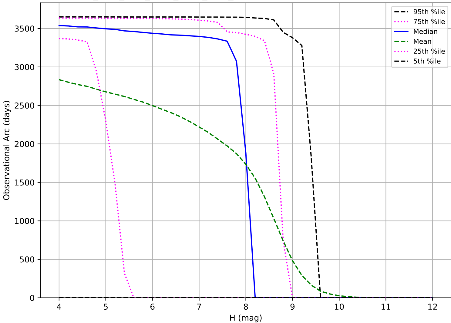
ddf_acor_sf15_Isf20_Isr10_v3.4_10yrs: Observational Arc Length TNO
