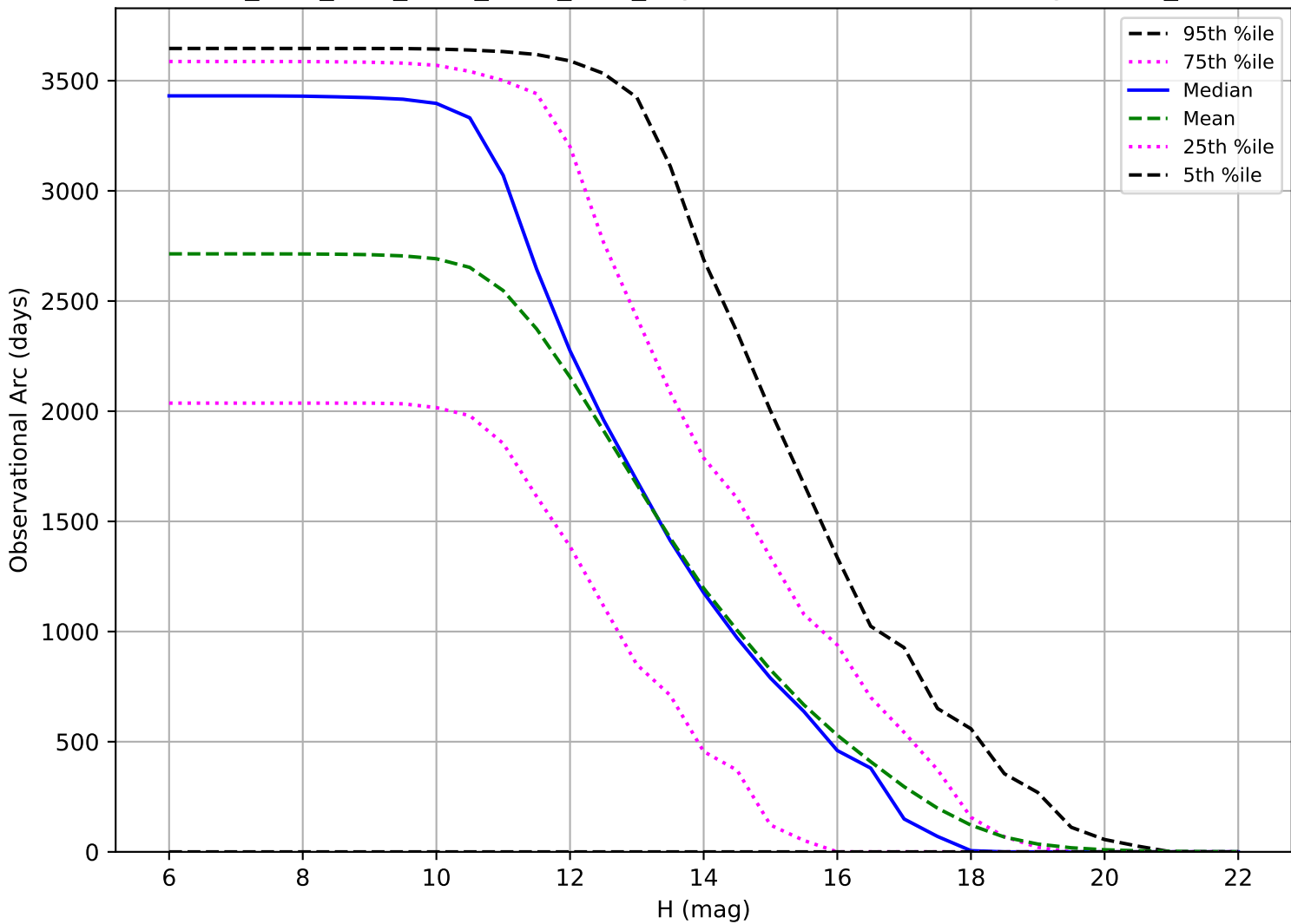
ddf_acor_sf15_lsf20_lsr10_v3.4_10yrs: Observational Arc Length OCC_r5
