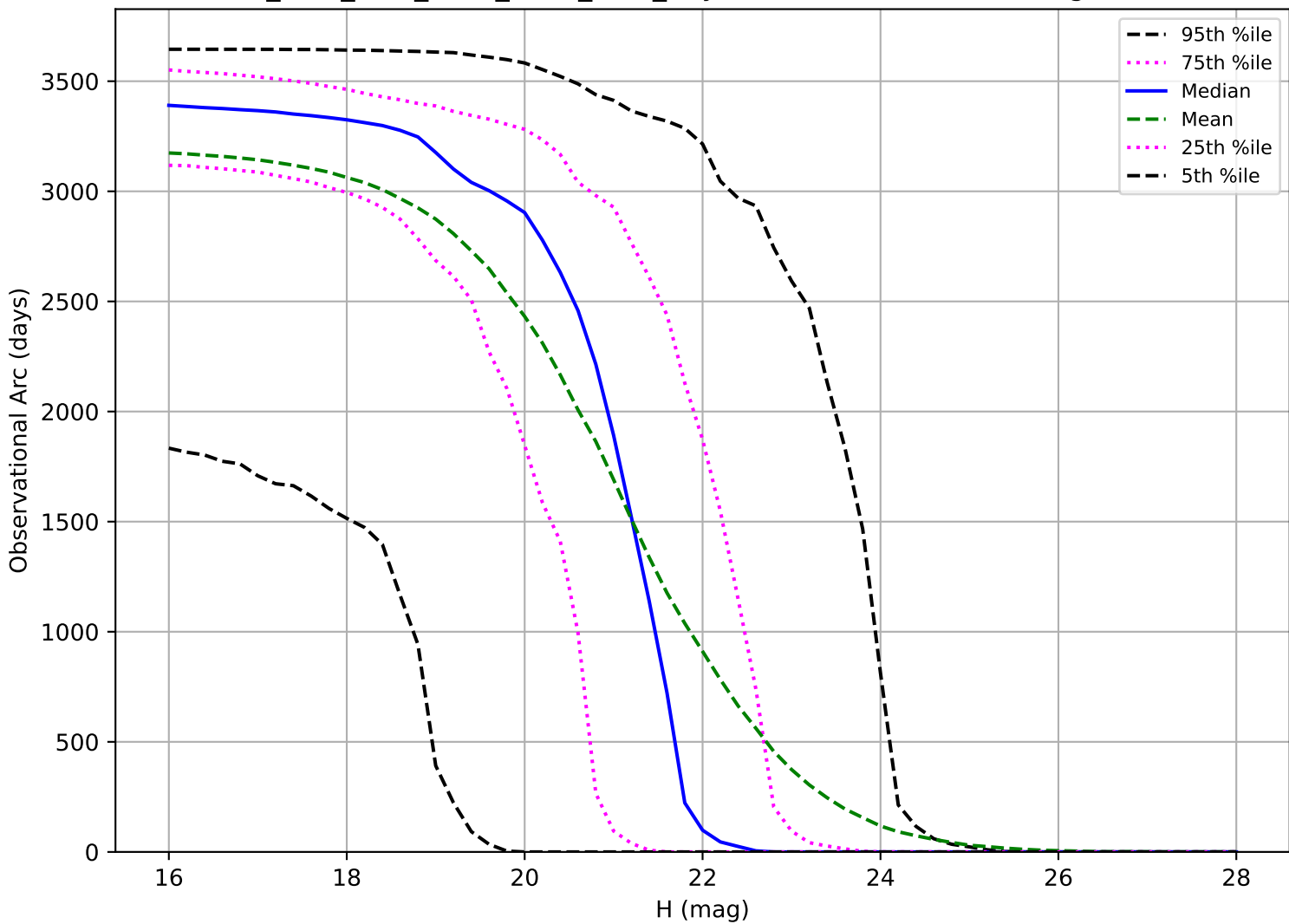
ddf_acor_sf15_lsf20_lsr10_v3.4_10yrs: Observational Arc Length NEO
