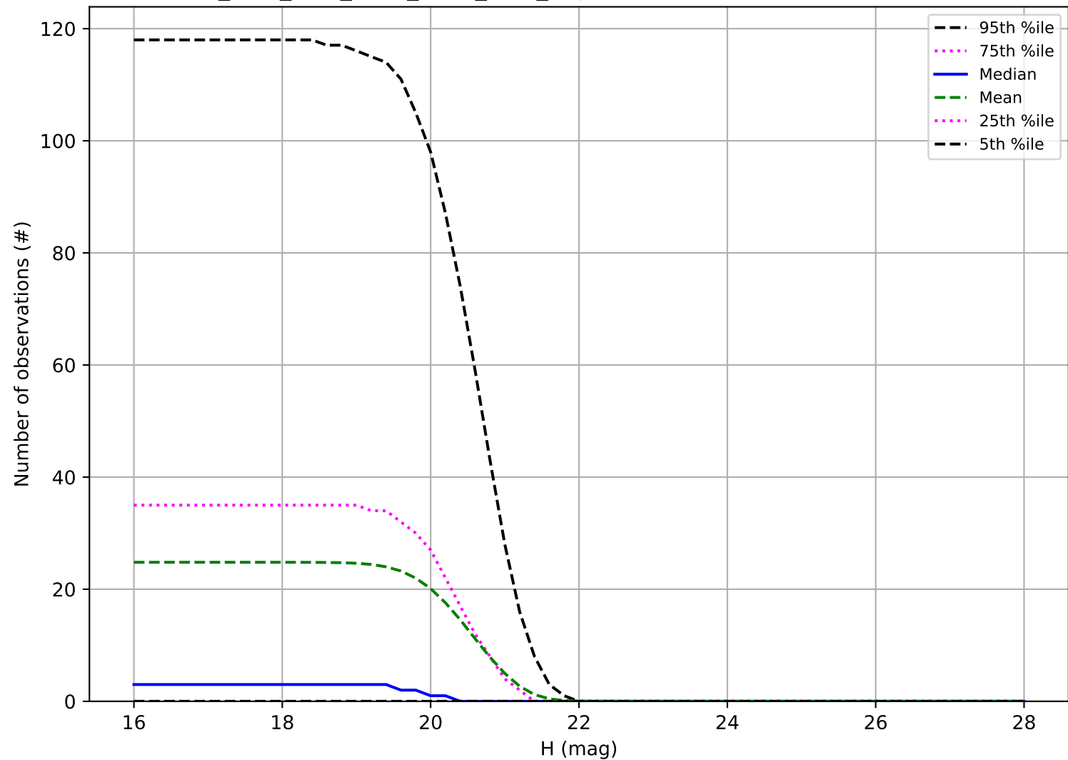
ddf_acor_sf15_lsf20_lsr10_v3.4_10yrs: Number of observations Vatira
