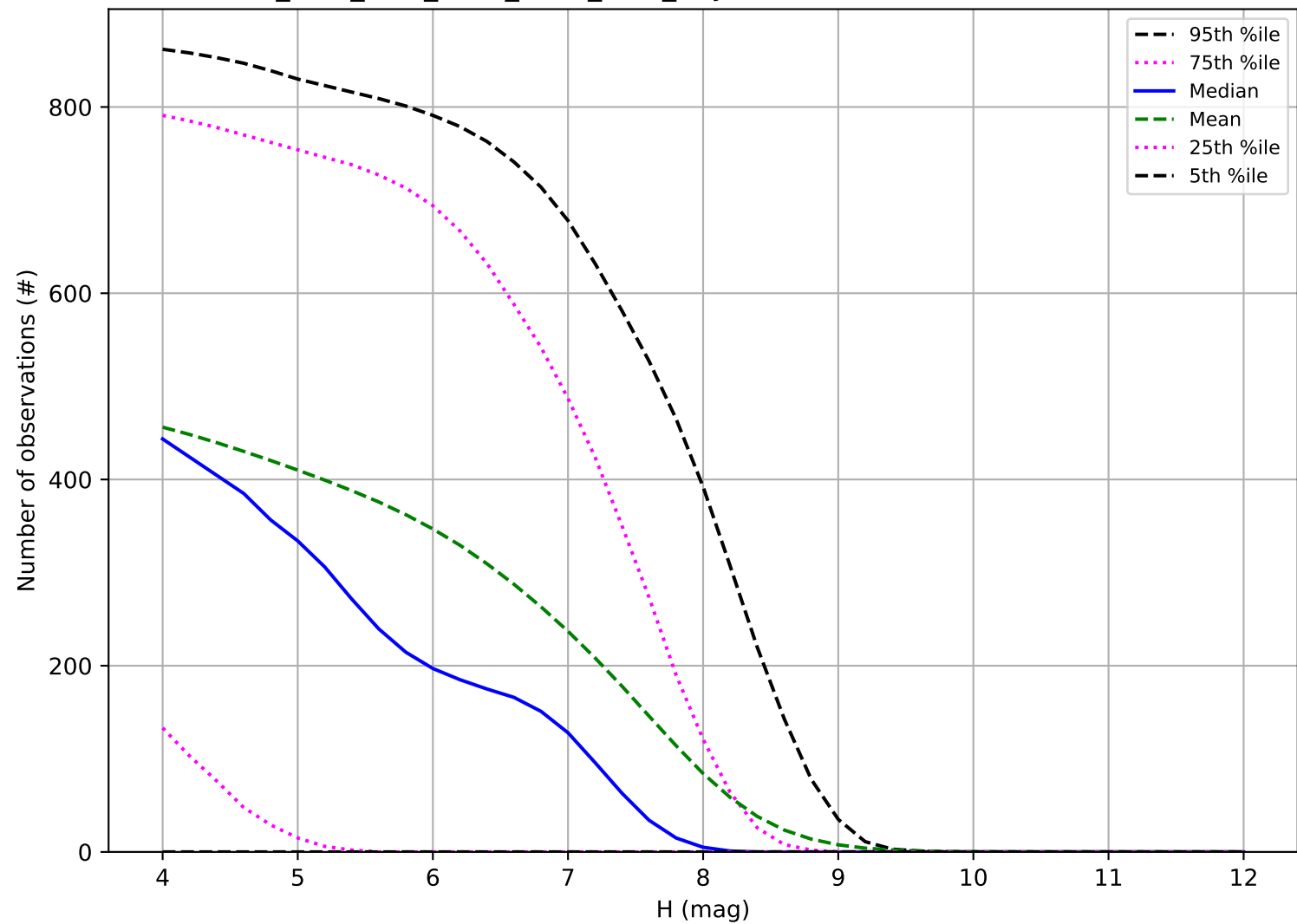
ddf_acor_sf15_lsf20_lsr10_v3.4_10yrs: Number of observations TNO
