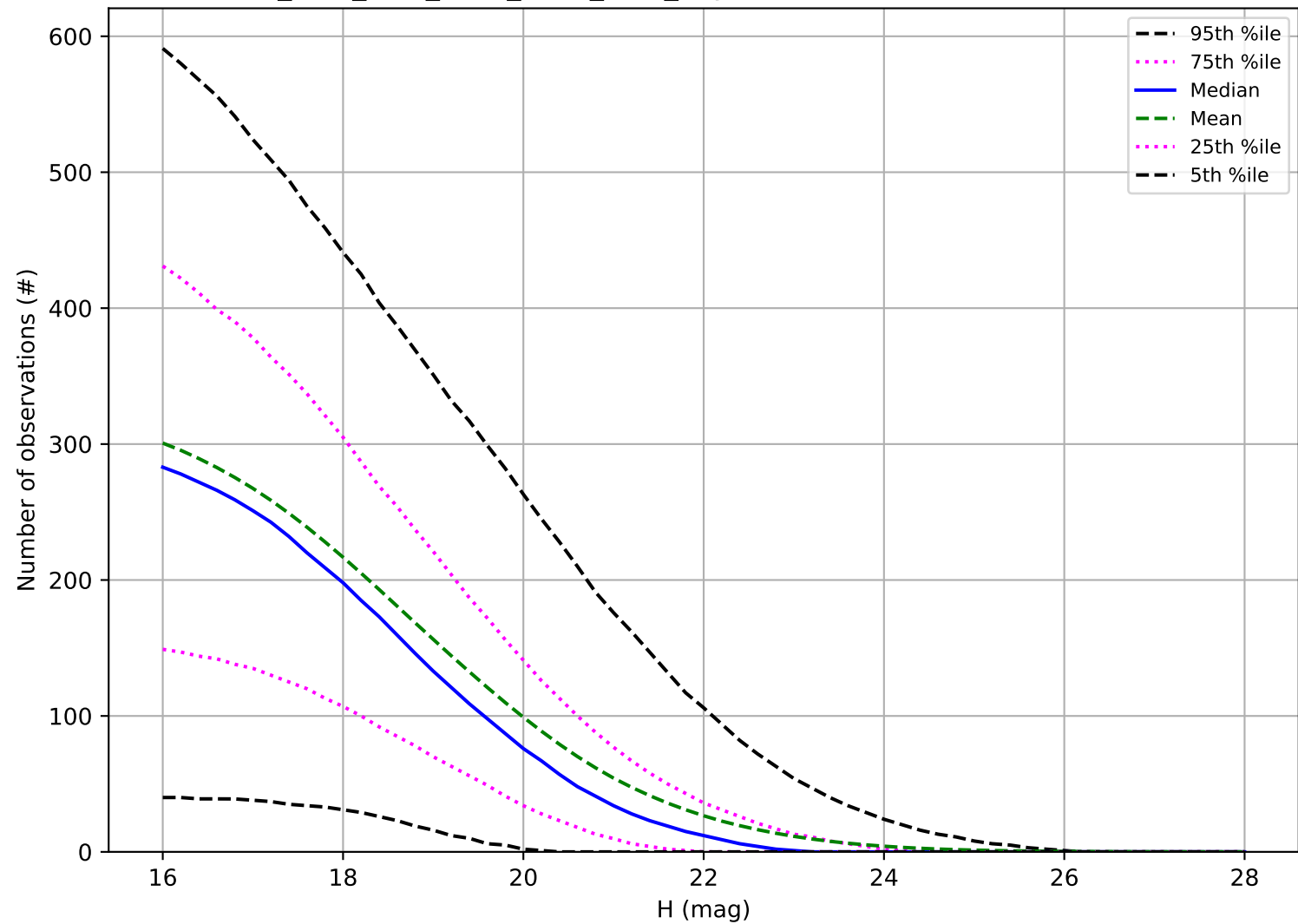
ddf_acor_sf15_lsf20_lsr10_v3.4_10yrs: Number of observations PHA
